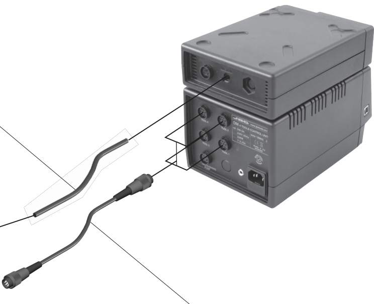
Stand cable extension Ref. A1286 Length: 1.5 m
