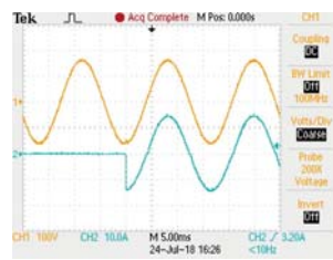
270 degrees loading
