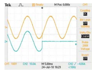
315 degrees unloading
