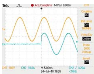
45 degrees loading
