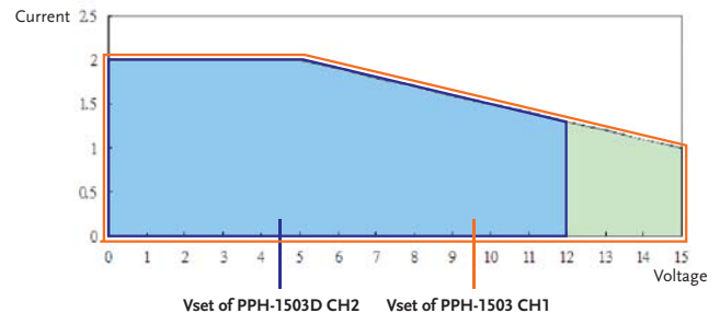
The Diagrams Show Voltage Setting Values and Allowable Sink Current for 3.5A and 2A of PPH-1503/PPH-1503D
