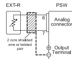
External Resistance control of the Voltage Output
