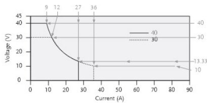
PSW 30V/40V Series Operating Area
