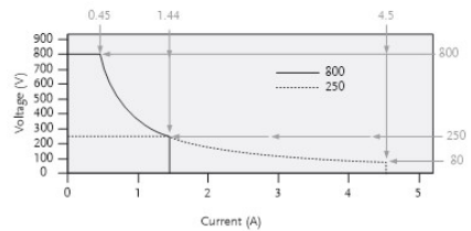
PSW 250V/800V Series Operating Area
