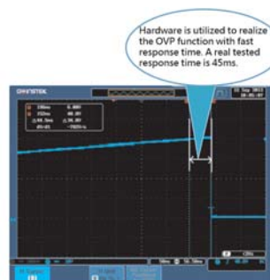
OVP Trigger
