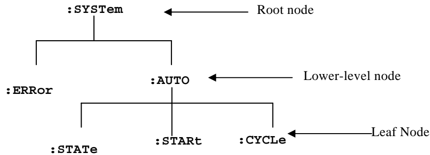
Figure 4: Tree hierarchy
