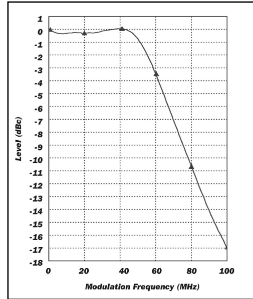
Typical AM Bandwidth
