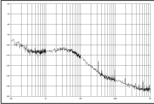
Typical SSB Phase Noise at 1 GHz
