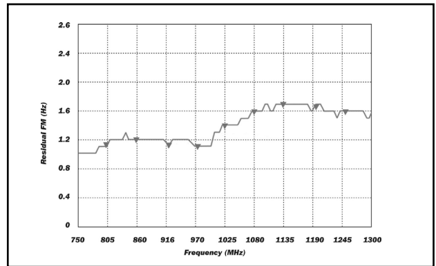
Typical Residual FM
