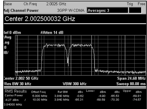
Typical 3GPP 2 carrier test model 1 (64 channels)
