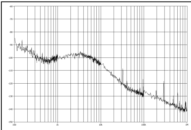
Typical Phase Noise at 2.1 GHz
