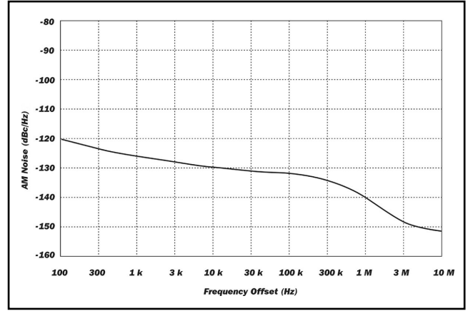
Typical AM Noise at 1 GHz
