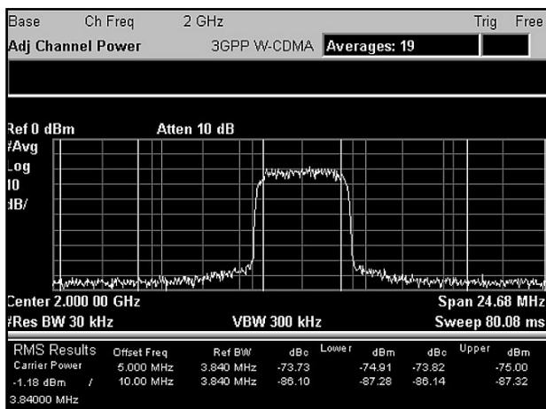
Typical 3GPP test model 1 (64 channels)
