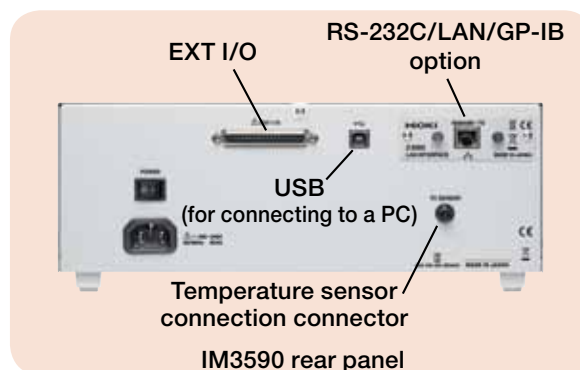
IM3590 rear panel
