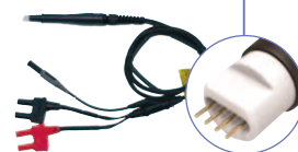
4-point probes (1.5 mm pitch)
