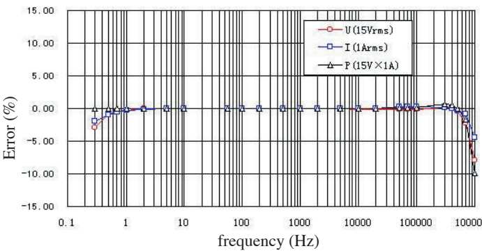
9600 Frequency characteristics (at 15V[15V×1A] range, response slow)
