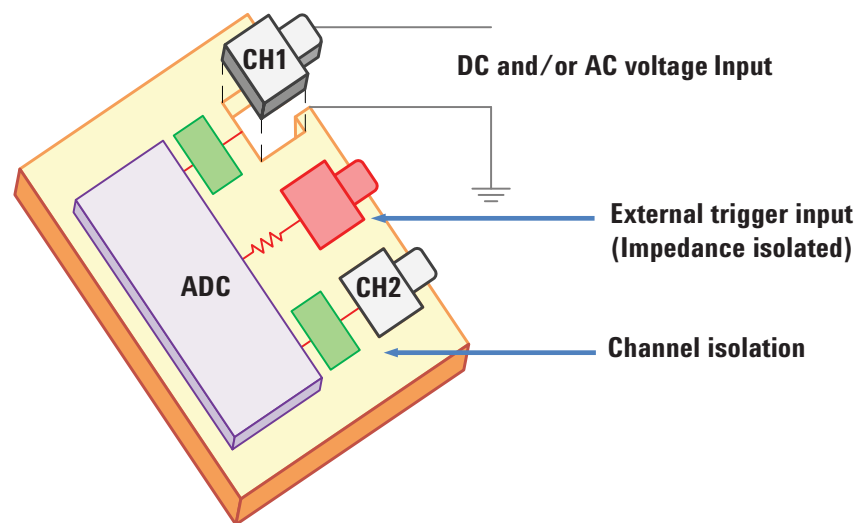
Figure 2. Isolated channel scope block diagram.
