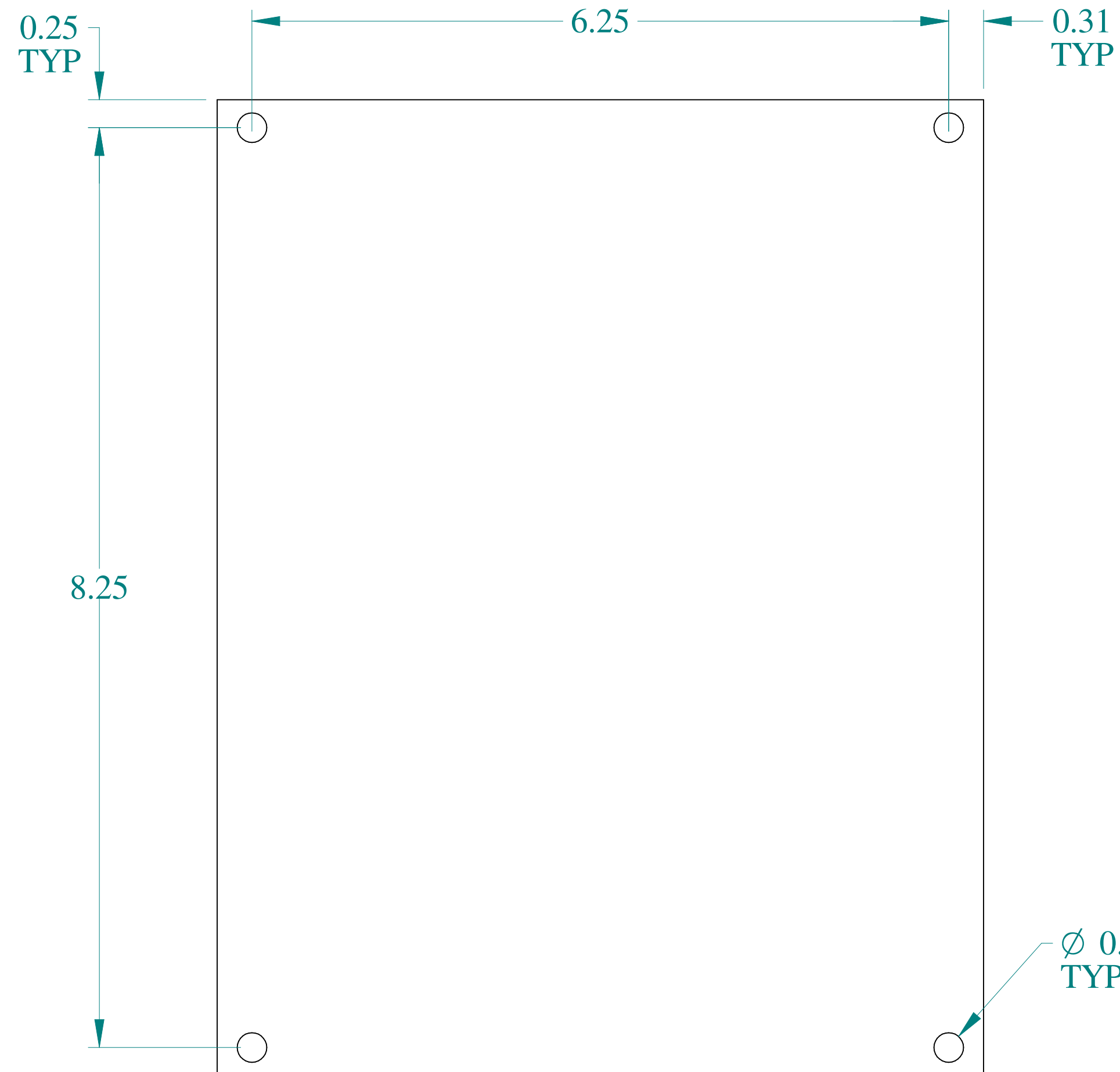
FRONT VIEW
