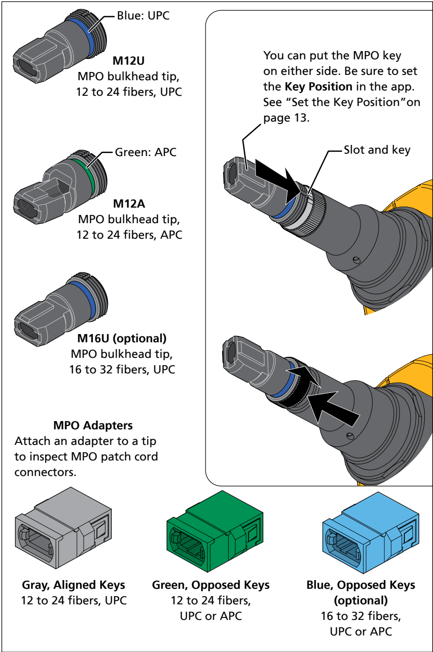
Figure 5. Tips and Adapters
