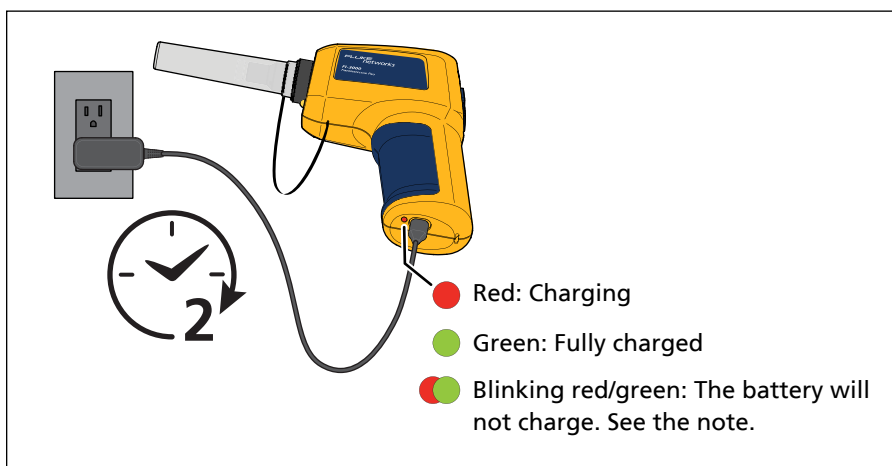
Figure 2. Charge the Battery Before You Use It
