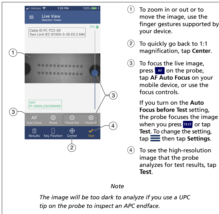
Figure 9. How to Adjust the Image
