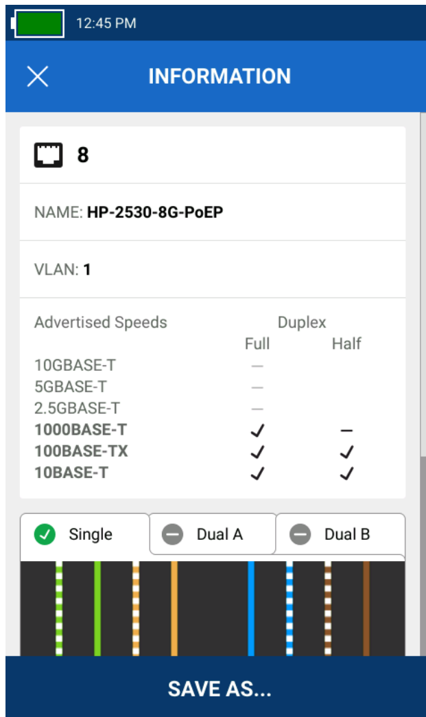
Switch port test shows port number, switch name and port VLAN along with advertised speed and duplex settings. Scrolling down shows Power over Ethernet Settings.
