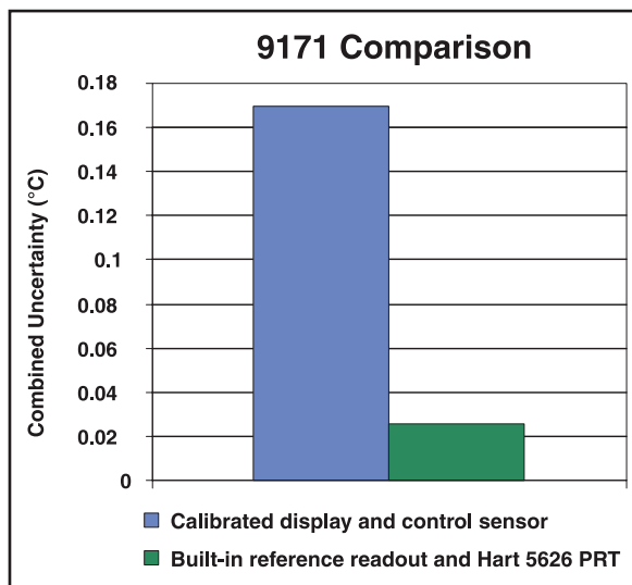
Figure 6. Total uncertainty is significantly reduced when using an external reference thermometer as the reference standard as shown above.
