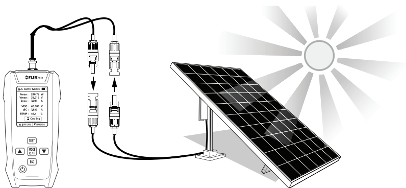
Figure 5.4 Connecting to solar panels and testing in automatic mode.
