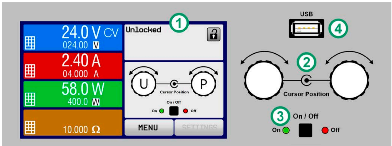
Figure 6- Control Panel
