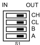
Figure 3. I/O module type switch (S1)
