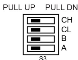
Figure 9. Switch S3 default configuration
