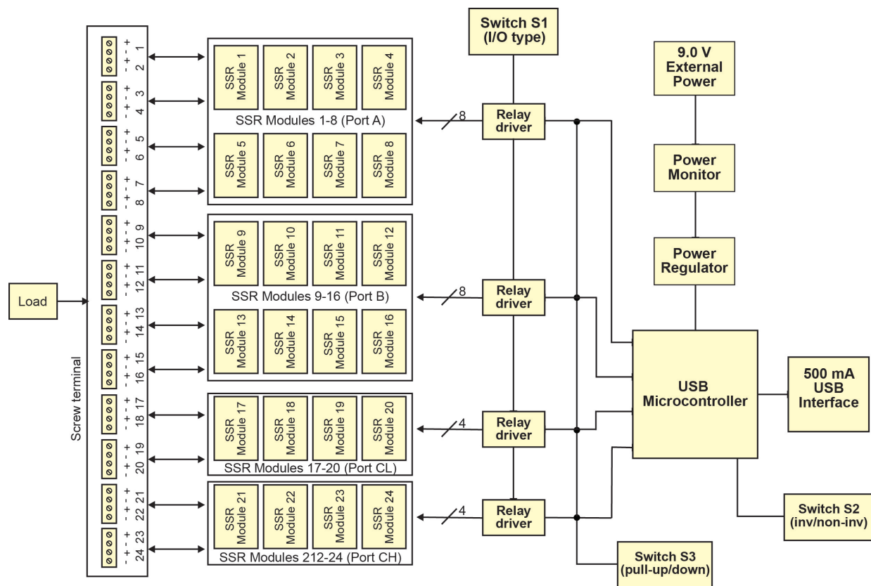
Figure 1. USB-SSR24 functional block diagram
