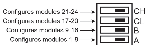
Figure 2. Typical PCB switch
