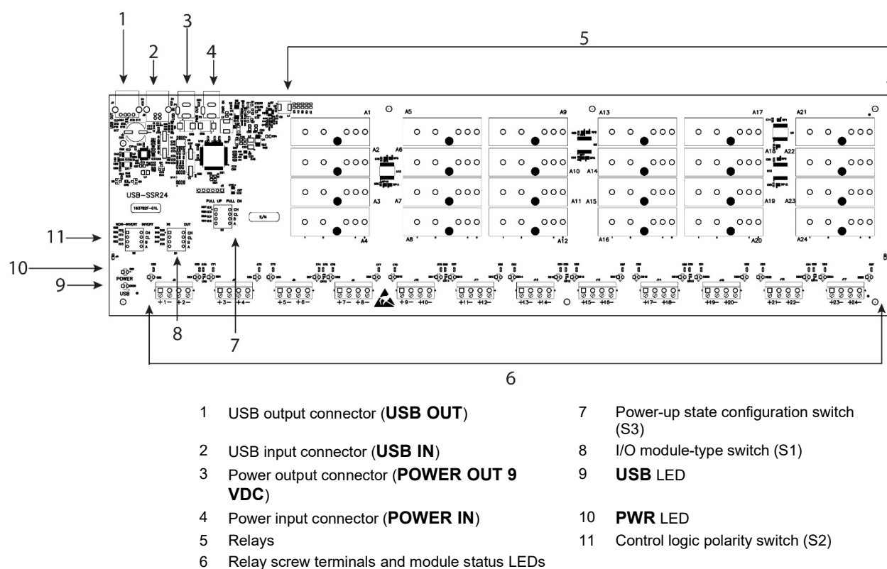
Figure 6. USB-SSR24 components
