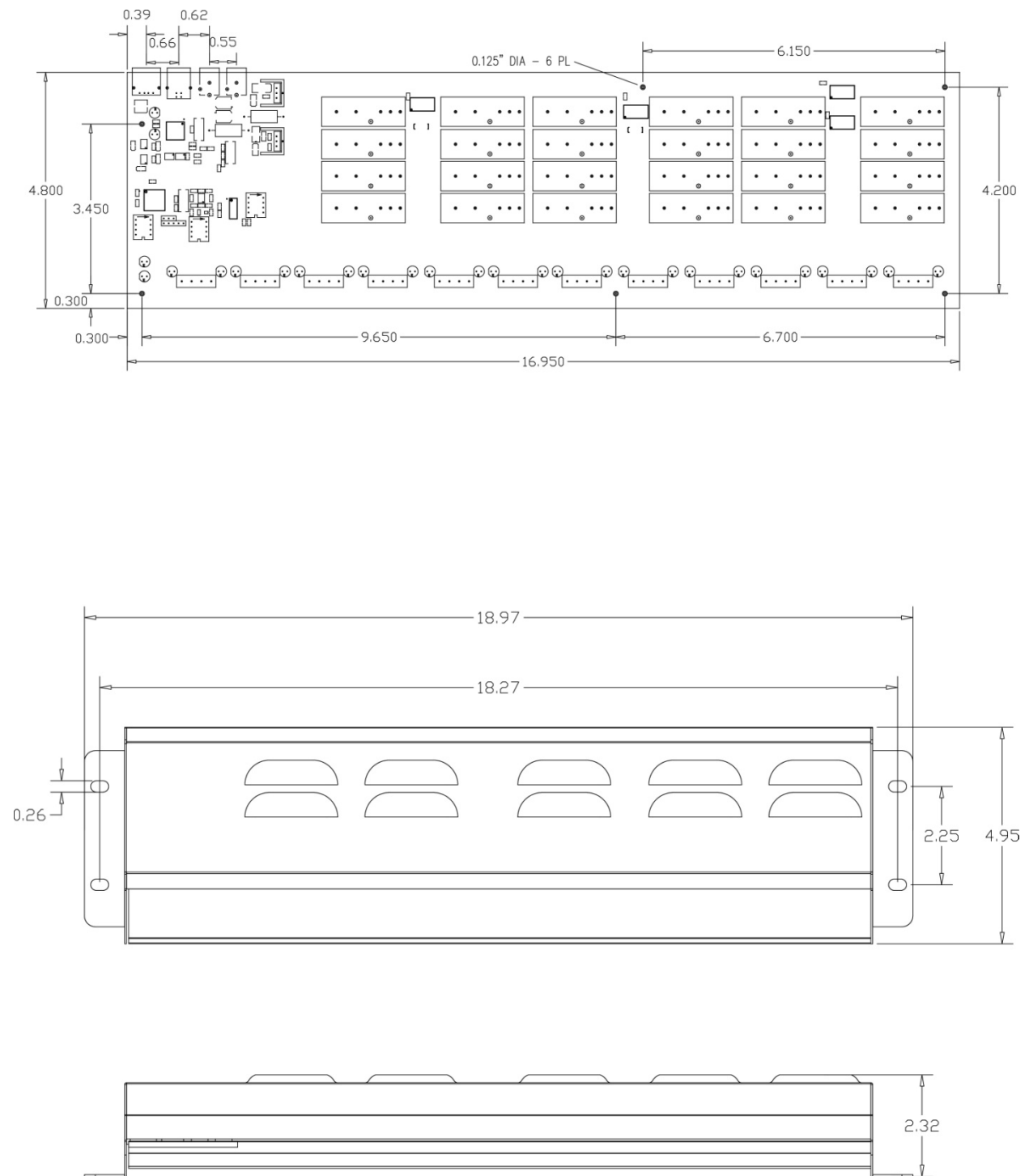
Figure 11. Circuit board (top) and housing dimensions
