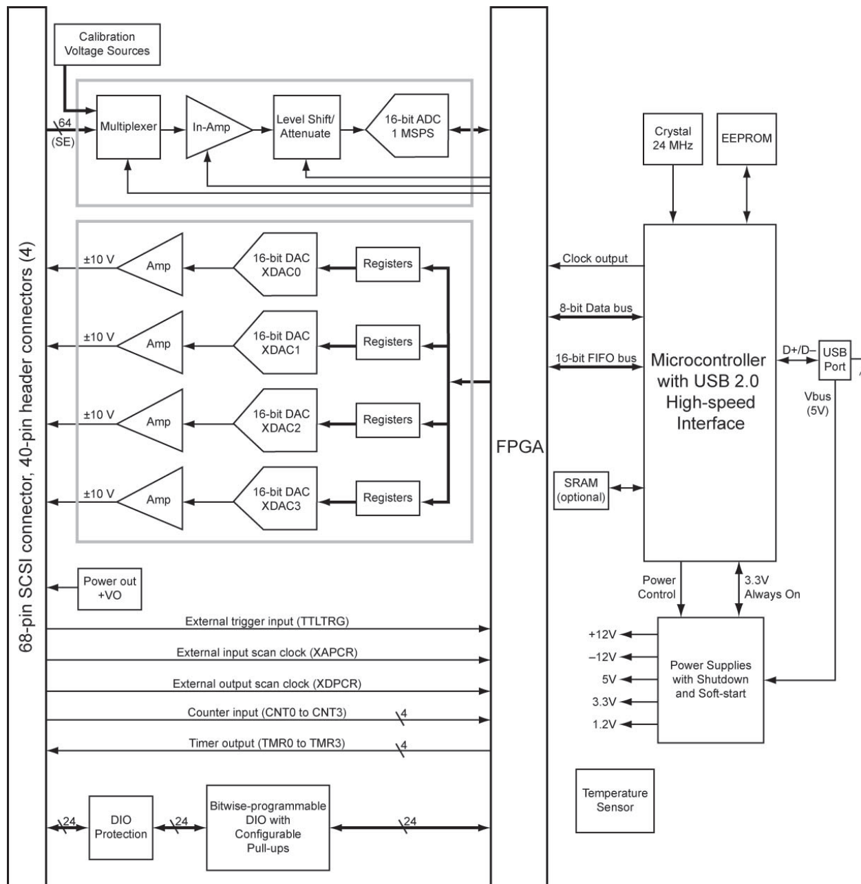
Figure 1. USB-2637 functional block diagram
