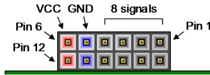
Figure 10.4.1: Pmod port
