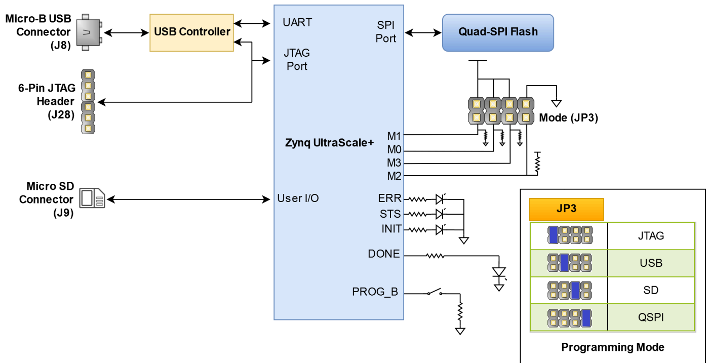
Figure 2.1: Genesys ZU Boot Diagram
