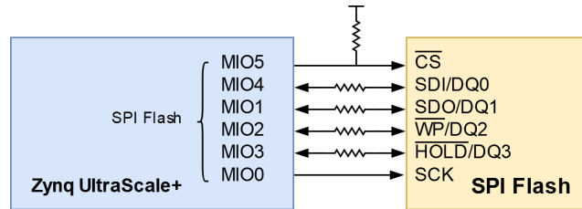
Figure 4.1.1: Genesys ZU Quad SPI Flash
