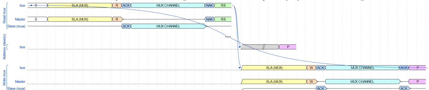
Figure 12.1.2: Genesys ZU I 2 C transfer format
