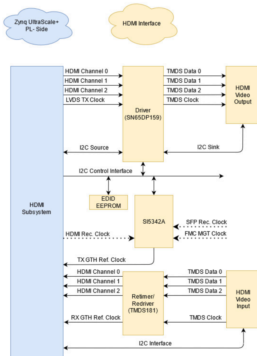
Figure 9.2.1: HDMI Interface Block Diagram
