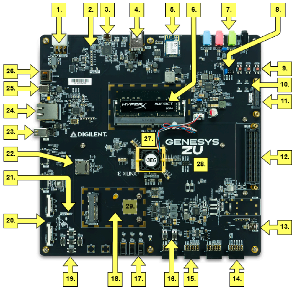
Figure 1: Genesys ZU-3EG callout diagram
