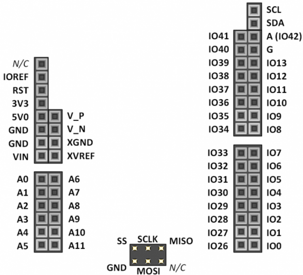
Figure 11.1 Arty A7 Shield Connector Pin Diagram
