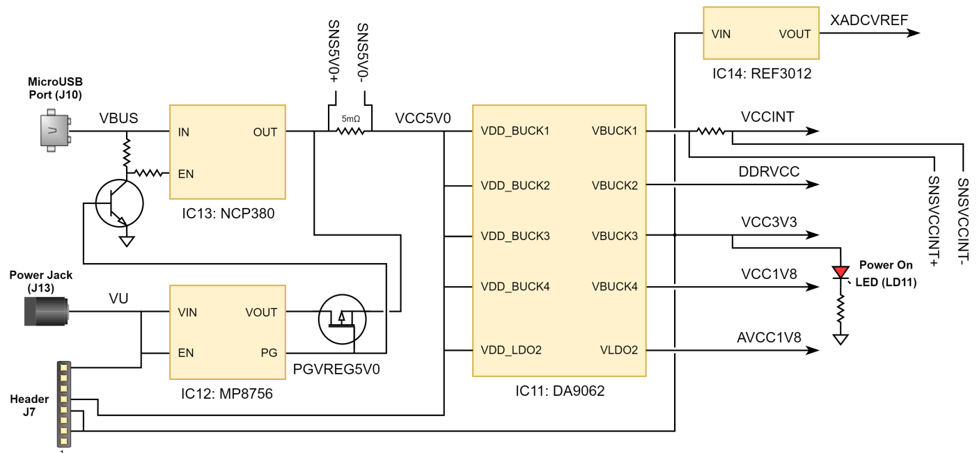
Figure 3.1 Arty A7 Power Circuit
