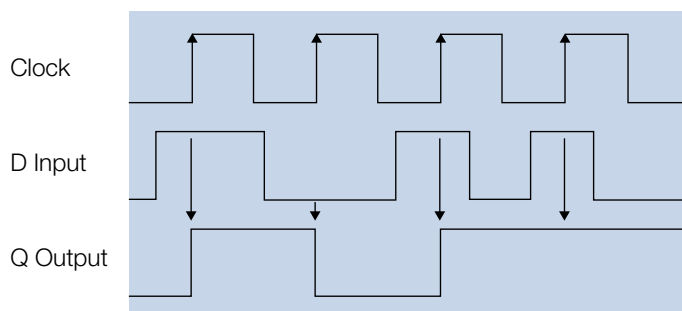
Figure 15. 74F74 D-Flip-Flop.
