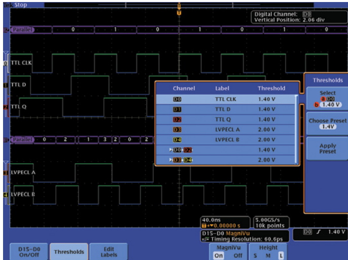
Figure 1. Mixed logic families (TTL & LVPECL) threshold settings on the same MSO4000B digital probe pod. The top three channels are TTL signals with a threshold of 1.40 V and the bottom two channels are LVPECL signals with a threshold of 2.00 V.
