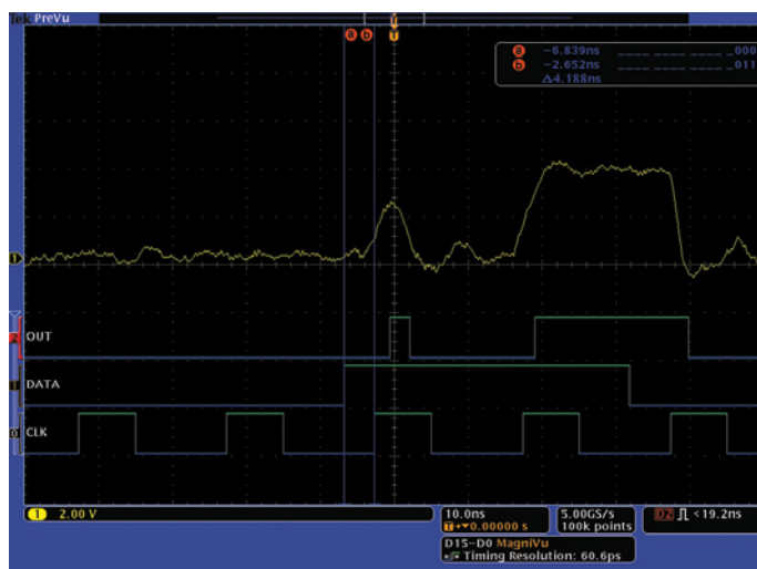
Figure 20. D-Flip-Flop Q output error with analog insight.
