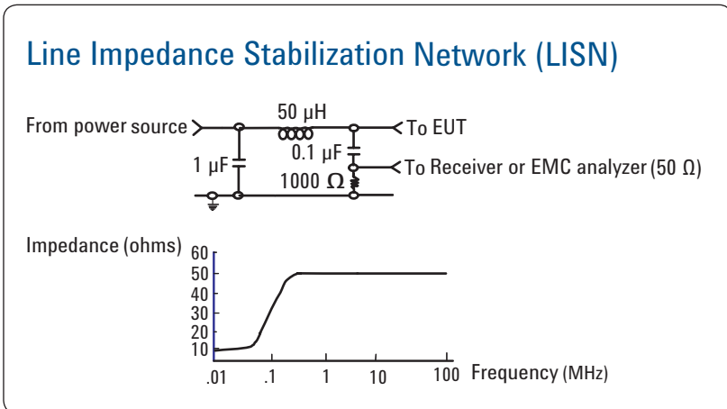
Figure A-1. Typical LISN circuit diagram
