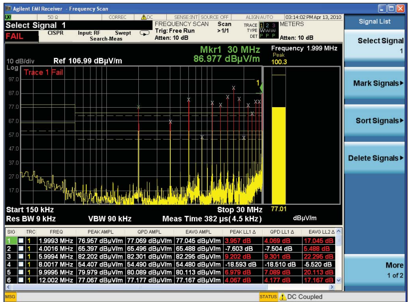
Figure 9. Quasi-peak and average delta to limit
