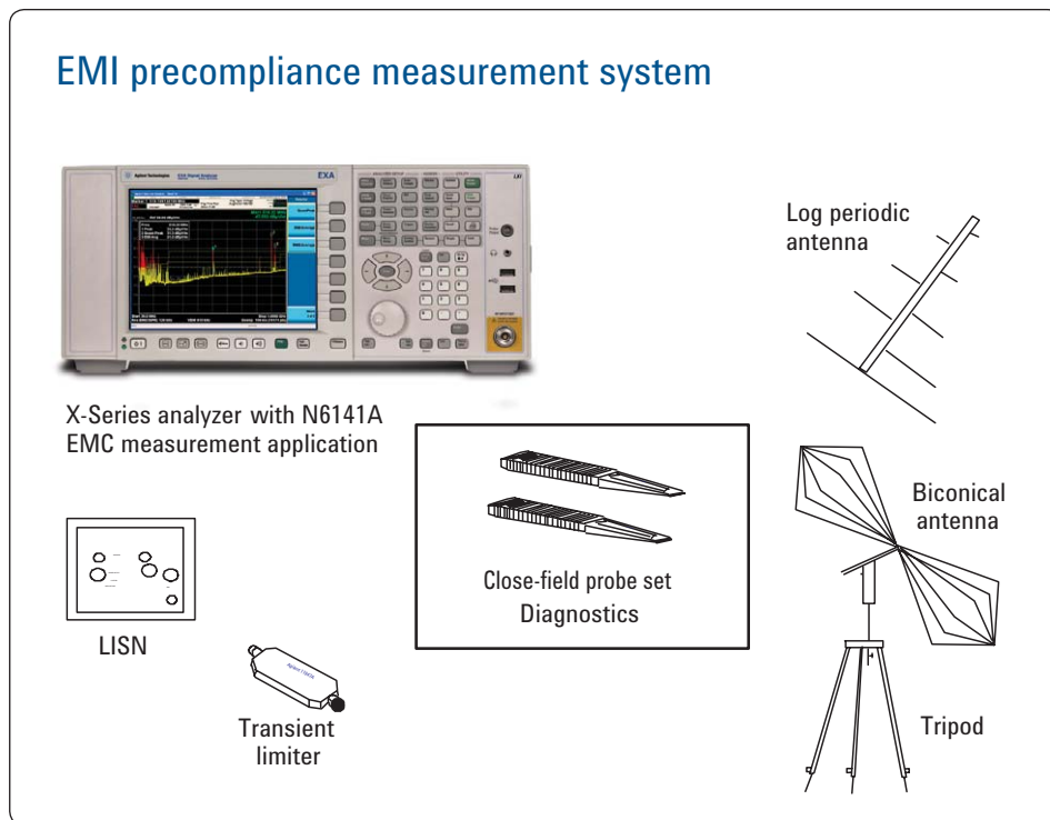
Figure 3. Components of a preproduction evaluation system
