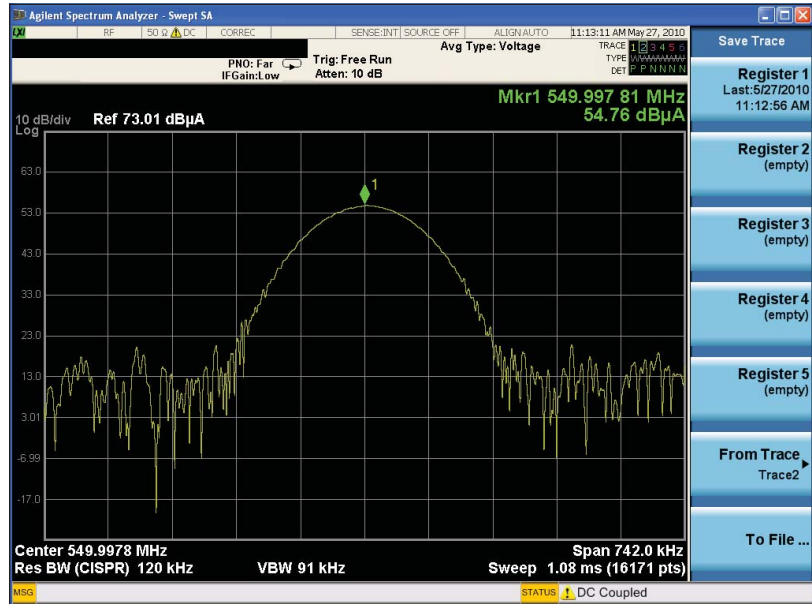
Figure 16. Preliminary diagnostics trace
