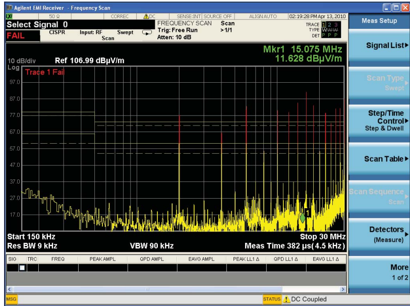
Figure 6. Conducted emissions display with limit lines and margin
