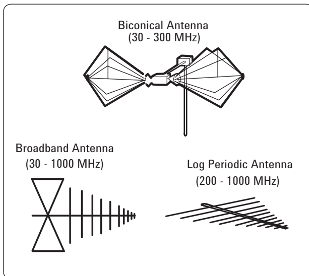
Figure B-2. Antennas used in EMI emissions measurements
