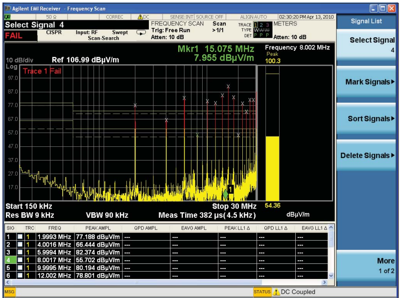
Figure 8. Scan and search for signals above the limit
