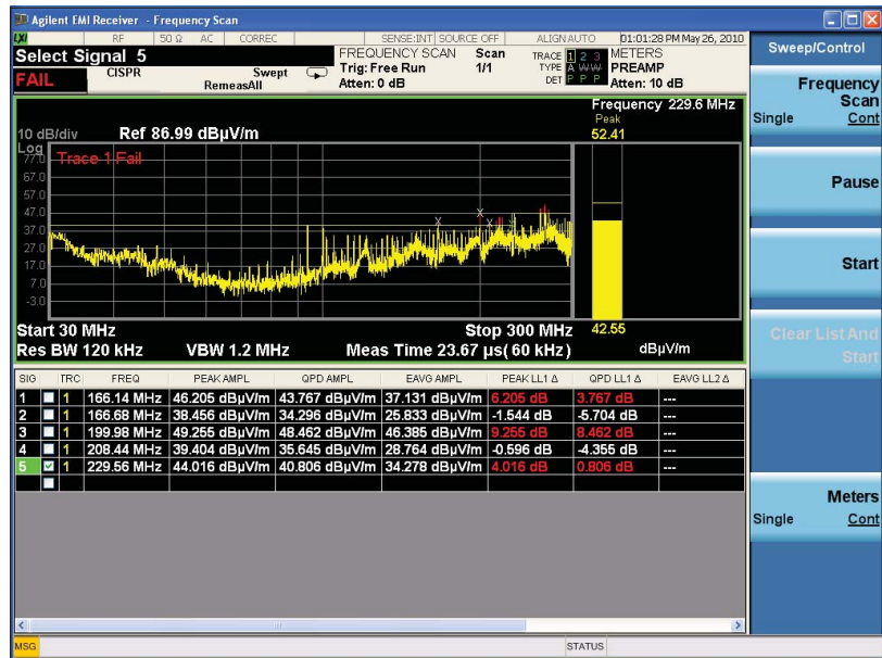
Figure 14. DUT signals with quasi-peak measurement compared to limit
