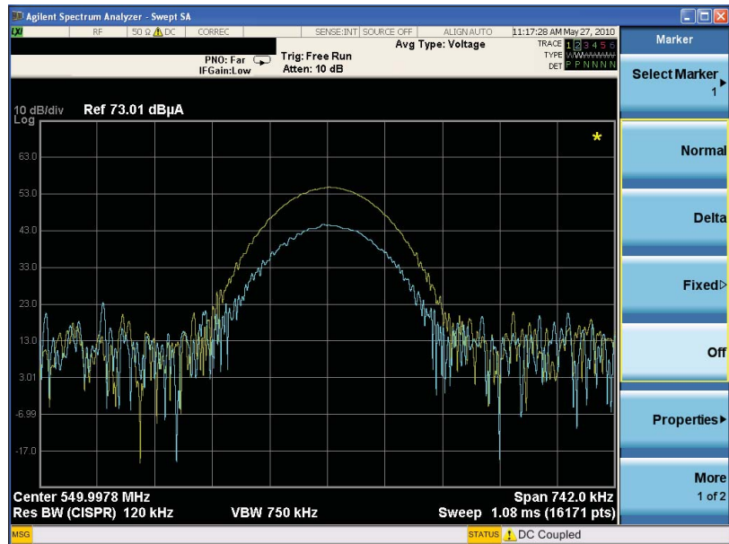
Figure 17. Diagnostics traces before and after redesign
