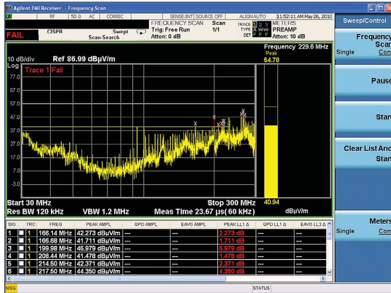
Figure 11. Ambient radiated emissions signals
