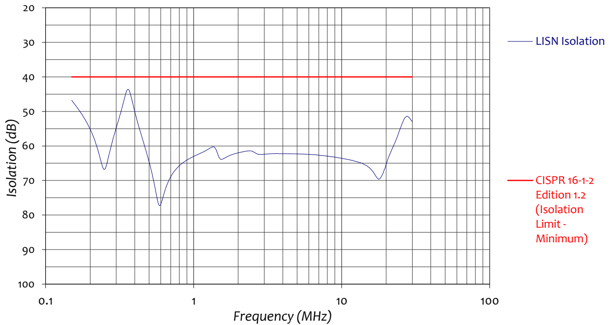
Figure 8: Typical Isolation compared to CISPR 16-1-2 requirements
