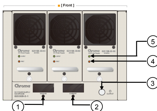
Figure 1-2 Front Panel of 62000B-3-1
