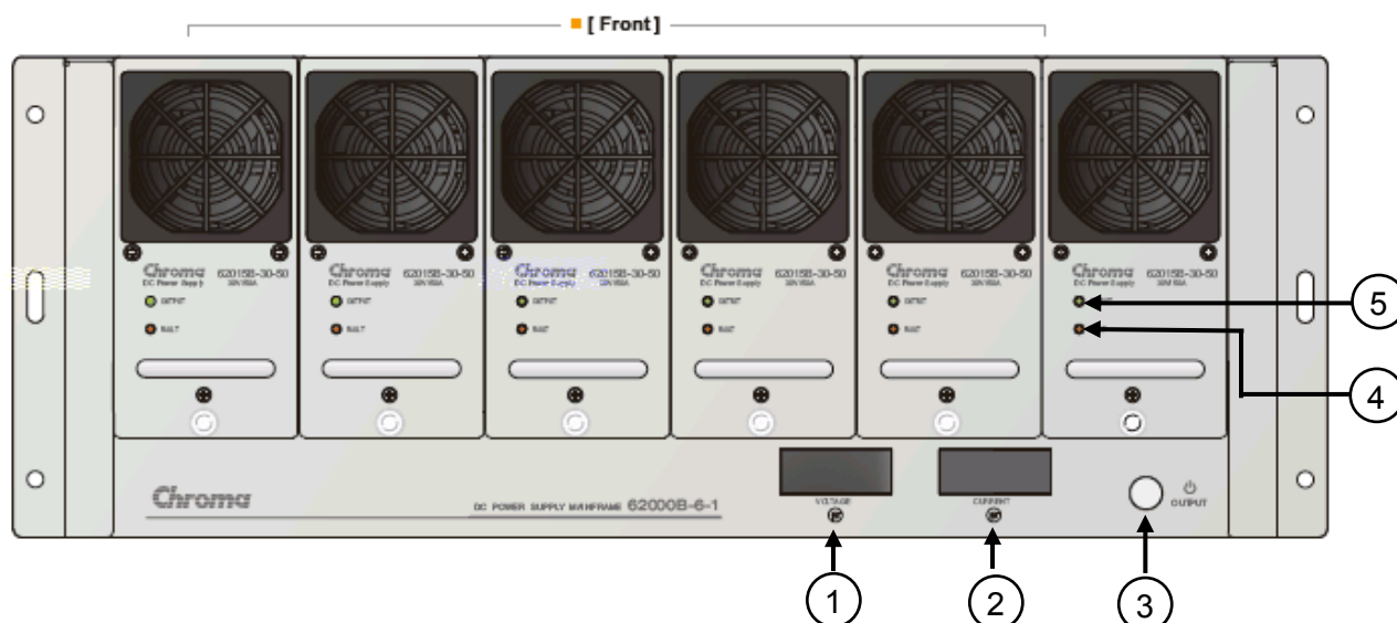
Figure 1-1 Front Panel of 62000B-6-1
