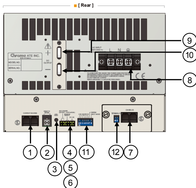
Figure 1-4 Rear Panel of 62000B-3-1
