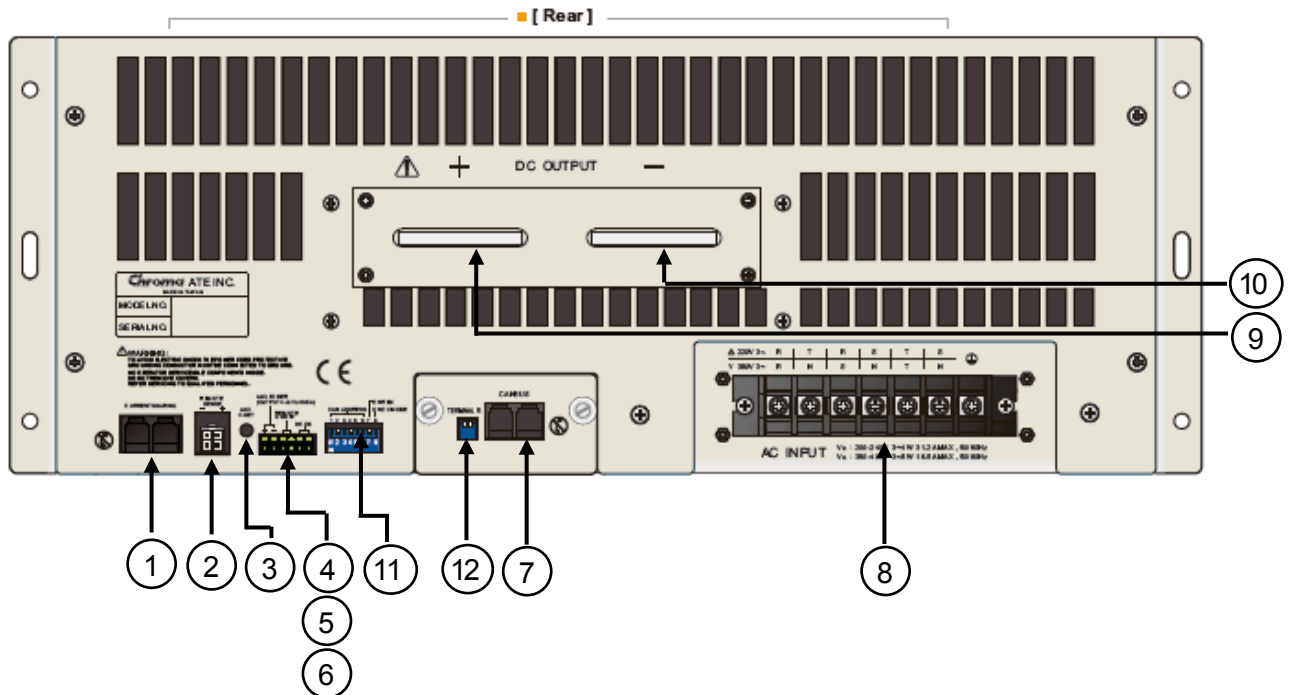
Figure 1-3 Rear Panel of 62000B-6-1
