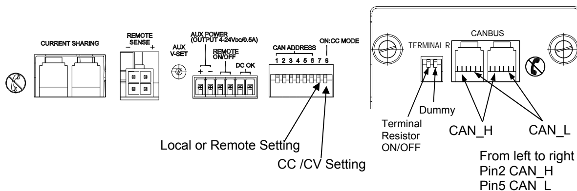
Figure 1-5 Communication Contacts on the Rear Panel
