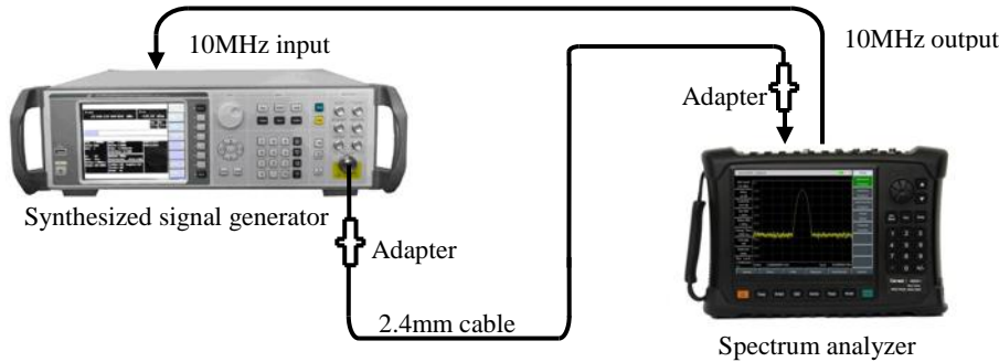
Fig. 12-6 Setting for Resolution Bandwidth Conversion Uncertainty
