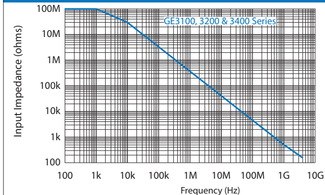
Figure 15: GE3000 Series Input Impedance Curve
