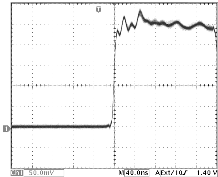
Figure 4 Rise Time 100x attenuation, 10%-90%
