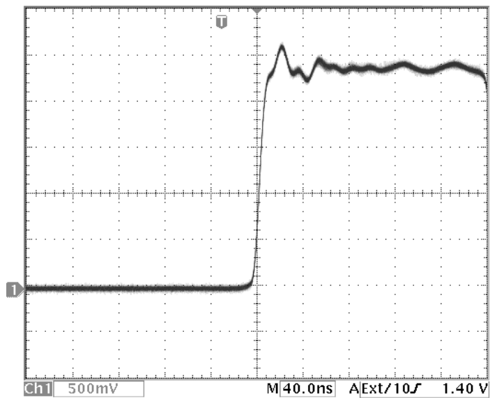
Figure 3 Rise Time 10x attenuation, 10%-90%
