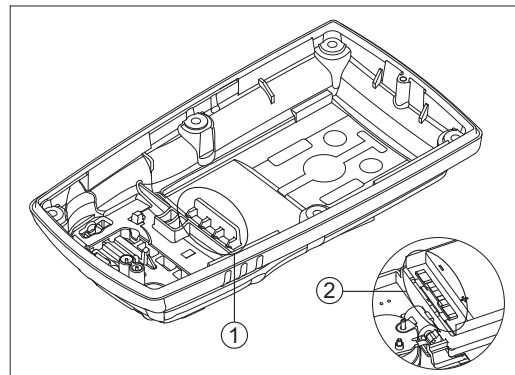
Figure 16. Replacing the Rear Shell
