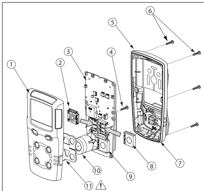
Figure 11. Replacing a Sensor or Sensor Filter
