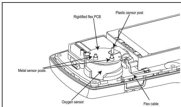
Figure 14. Replacing the Oxygen Sensor for XT and XL
