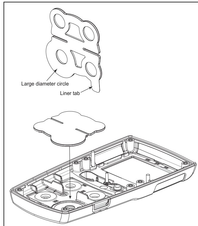
Figure 12. Liner Tab
