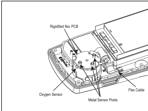
Figure 15. Replacing the Oxygen Sensor for X3
