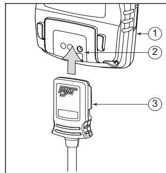
Figure 9. Connecting to the IR Link
