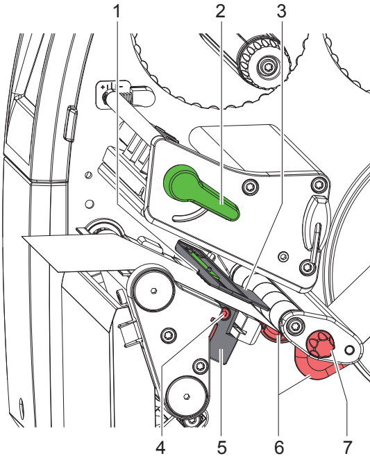
Figure 12 Inserting the media strip into the printhead
