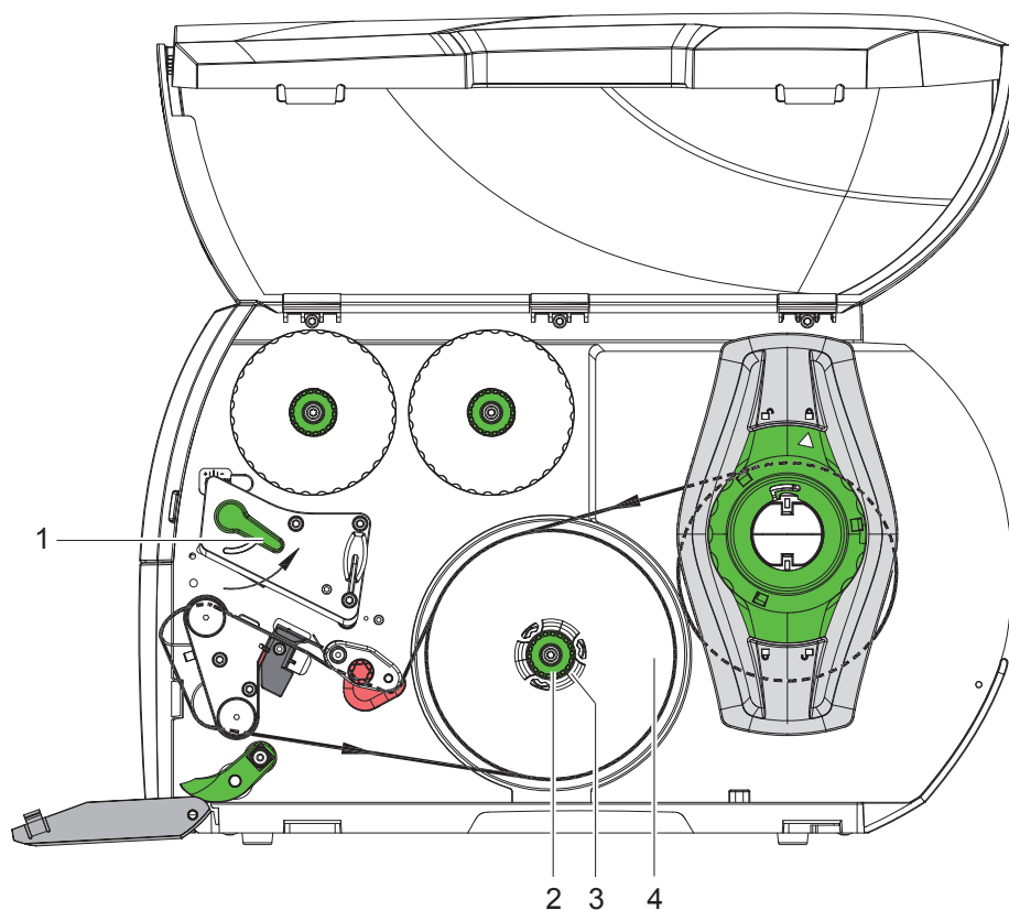
Figure 14 Removing the wound roll
