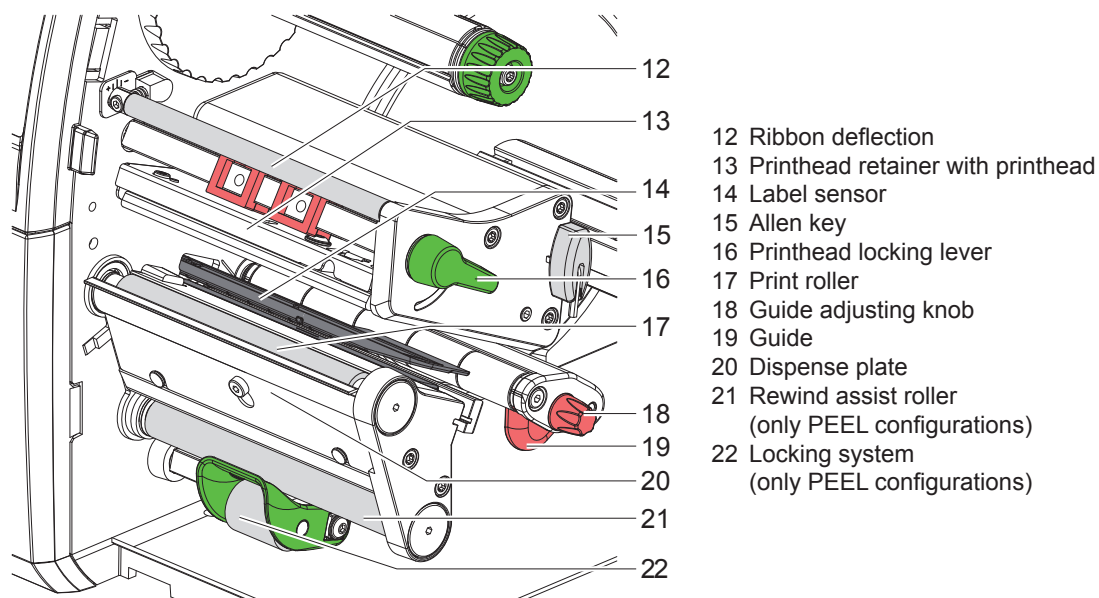
Figure 2 Print unit
