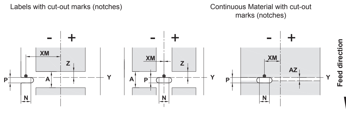
Figure 27 Cut-out mark dimensions
