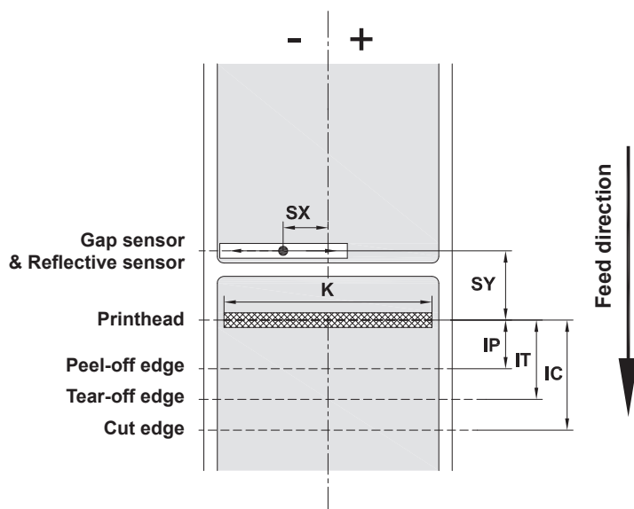
Figure 25 Device dimensions
