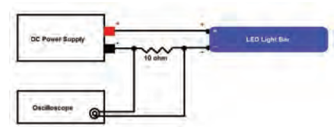
Example LED test setup
