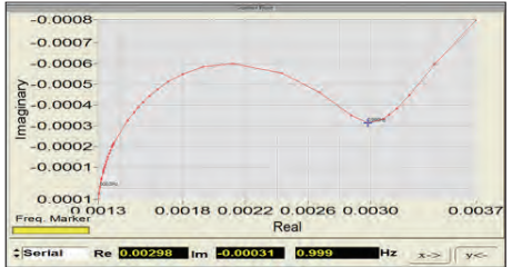
Nyquist diagram
