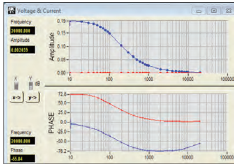
V/I plot
