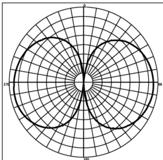
M401 (900 MHz, E plane)
