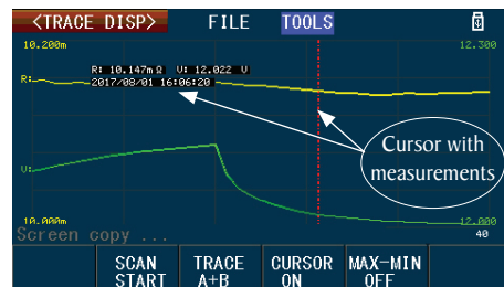
Trace display
