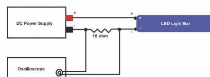
Example LED test setup
