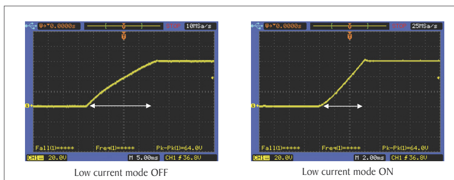
Voltage rise time with and without low current mode enabled
