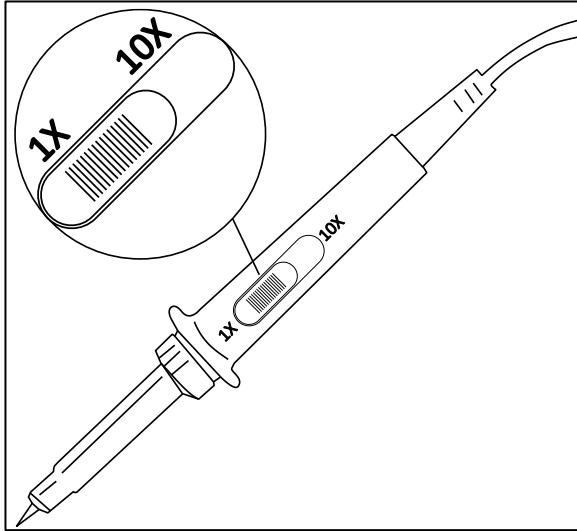
Figure 2.5 – Oscilloscope Probe
