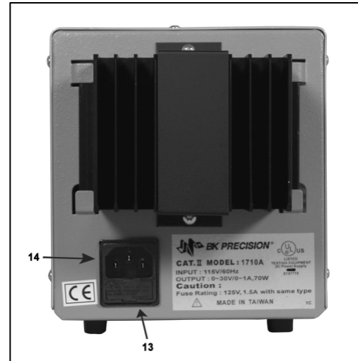
Figura 2. Panel trasero
