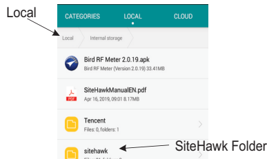
Figure 40 Folder Navigation
