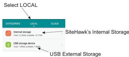
Figure 39 File Selection
