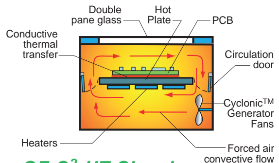
GF-C²-HT Chamber
