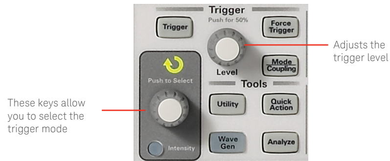
Figure 20. Front panel trigger control section on a Keysight InfiniiVision 2000 X-Series oscilloscope
