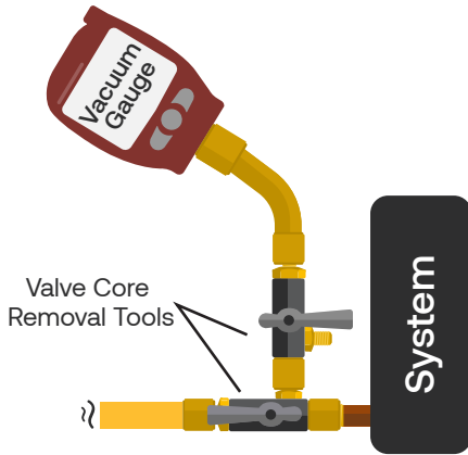
(Setup shown isolates AV760 during charging)
