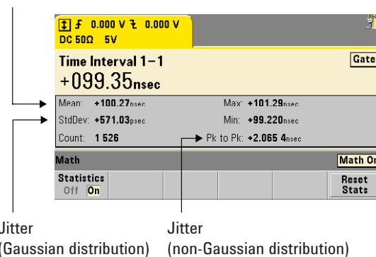
FIGURE 4: 5320A display with statistics enabled
