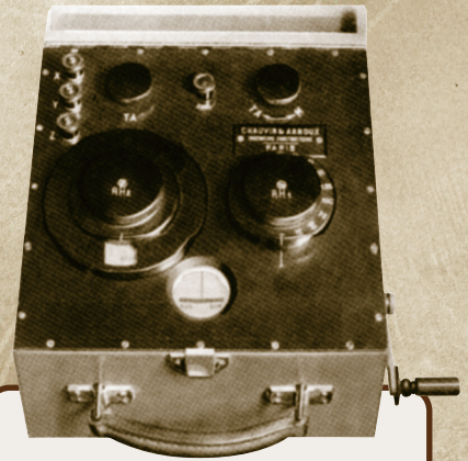
First Ground Tester introduced in 1935
