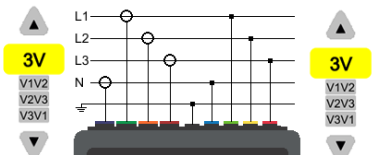
Three-phase 5 wires (L1, L2, L3, N, and earth)
