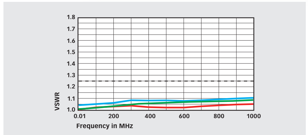
Typical VSWR — ATN 6060, — ATN 6150, — ATN 6200, - - - limit
