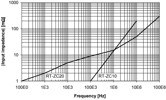
Insertion impedance (meas.).
