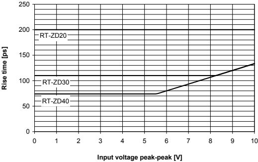
R&S®RT-ZDxx rise time (meas.).
