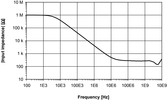
R&S®RT-ZS60 input impedance versus frequency.
