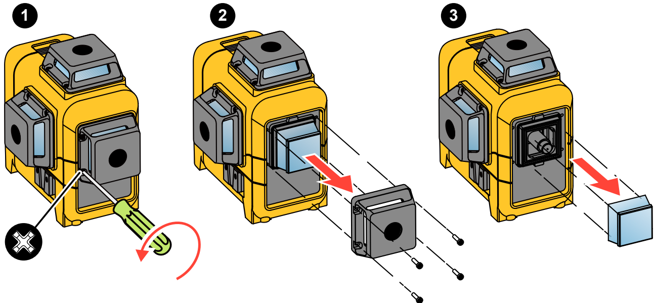
Figure 4. Housing Glass Insert Replacement
