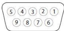
Figura 2-1 Pins RS232
