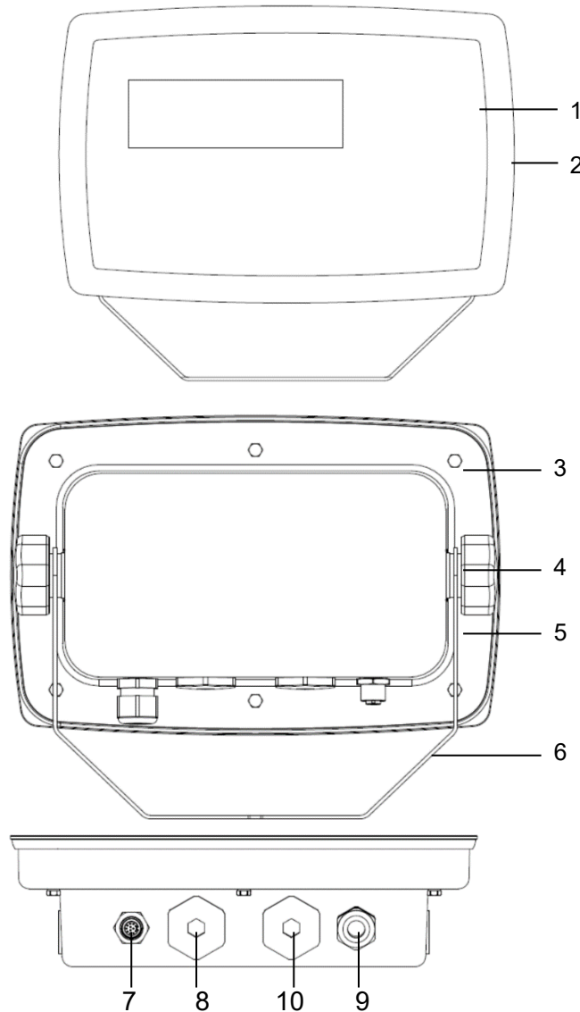
Figure 1-2 TD52XW Indicator
