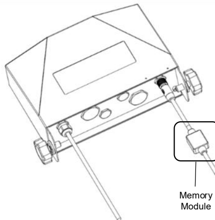
Figure 7-5. Connecting cable with connector and memory module
