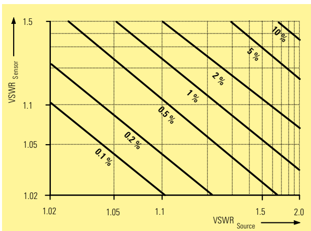
Limits of power measurement error caused by mismatch of sensor and signal source
