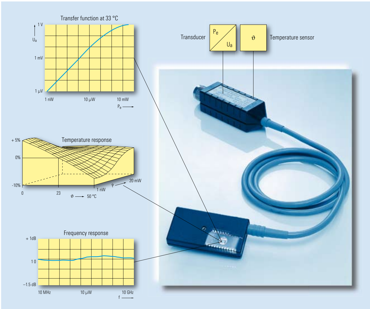
The individual calibration data is stored in a non-volatile memory in the connector of each sensor
