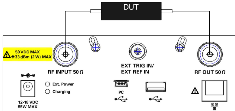
Figure 2 Transmission coefficient measurement setup
